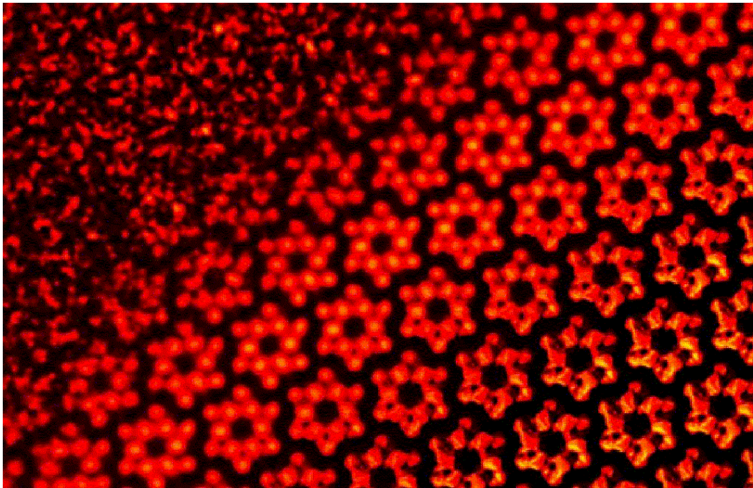
The asymmetric membrane of the urea bladder (from top left to down right : Original data; 2D reconstruction; 3D reconstruction)
